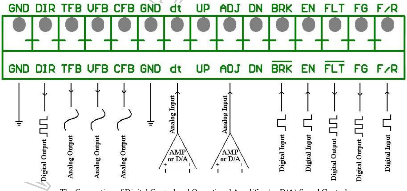
The Connection of Digital Control and Operational Amplifier (or D/A) Speed Control
